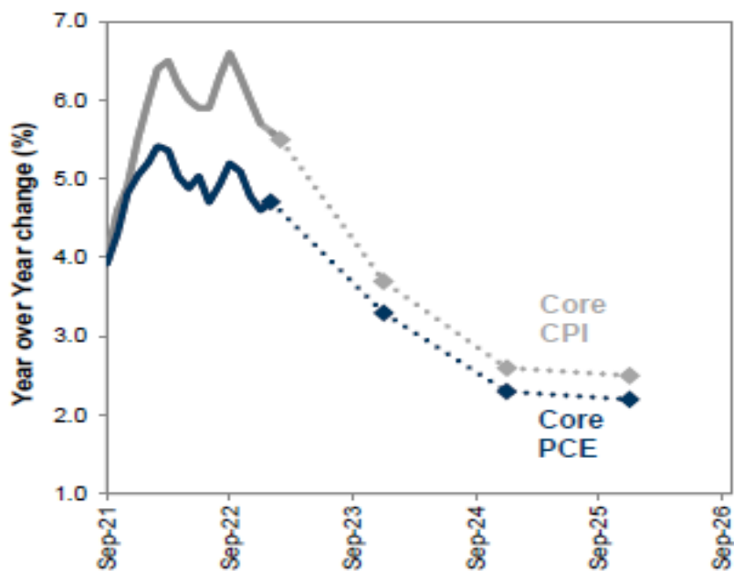
Core PCE and CPI
